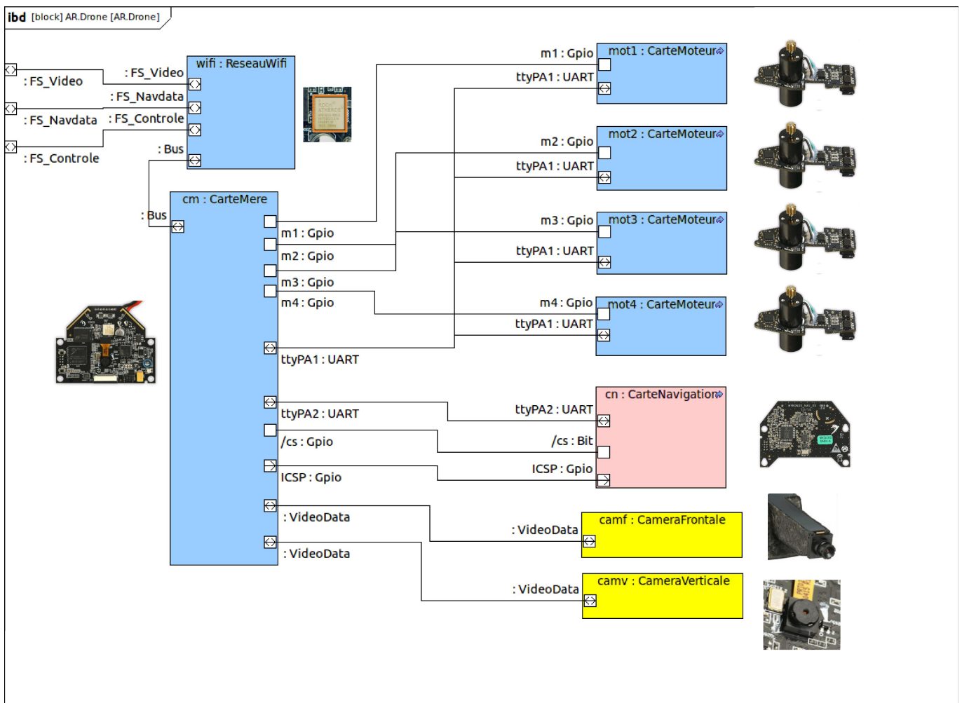
Fig. 49: IBD AR.Drone
