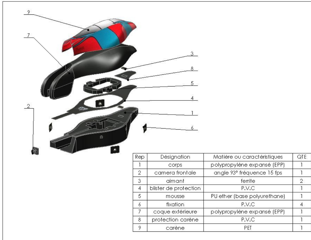
Fig. 61: Chassis AR.Drone
